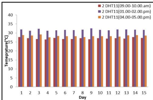
Figure 15. Graph of temperature of the second sensor
